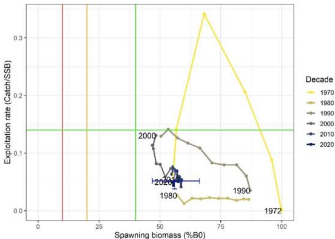
Figure 29: Trajectory over time of exploitation rate (U) and spawning biomass (% B0), for the LIN 3&4 base model from the start of the assessment period in 1972 to 2022. The red vertical line at 10% B0 represents the hard limit, the orange line at 20% B0 is the soft limit, and green lines are the % B0 target (40% B0) and the corresponding exploitation rate ( U_{40} = 0.14 calculated using CASAL CAY function). Biomass and exploitation rate estimates are medians from MCMC posteriors for the base model. The blue cross represents the limits of the 95% confidence intervals of the estimated ratio of the SSB to B0 and exploitation rate in 2022.
