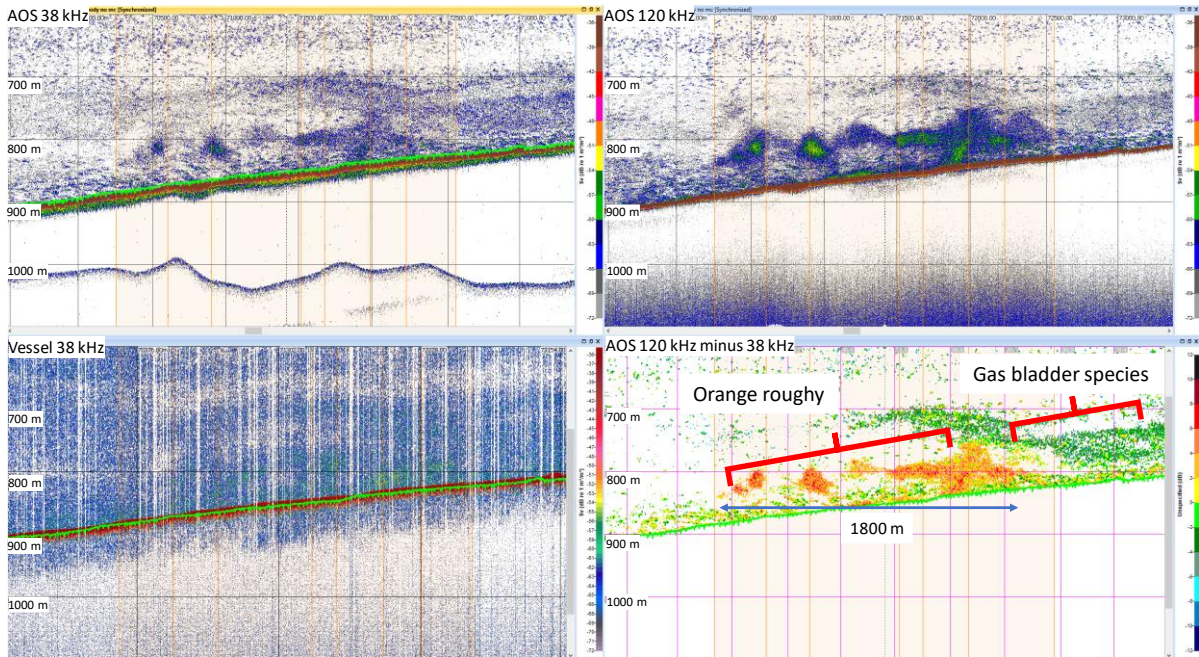
Figure 8. Example of multifrequency echograms from a Sealord AOS transect at Rekohu in July 2021 (top panels). Bottom left panel shows the echogram from the Amatal Apollo's 38 kHz echosounder.
