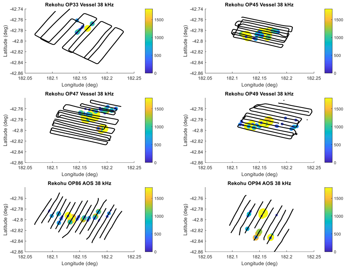
Figure 52. Map of biomass surveys at Rekohu with circle size indicating backscatter (NASC) value for each echointegration interval. Bubble size is scaled by the largest NASC value for the surveys. Colour bar indicates NASC values.
