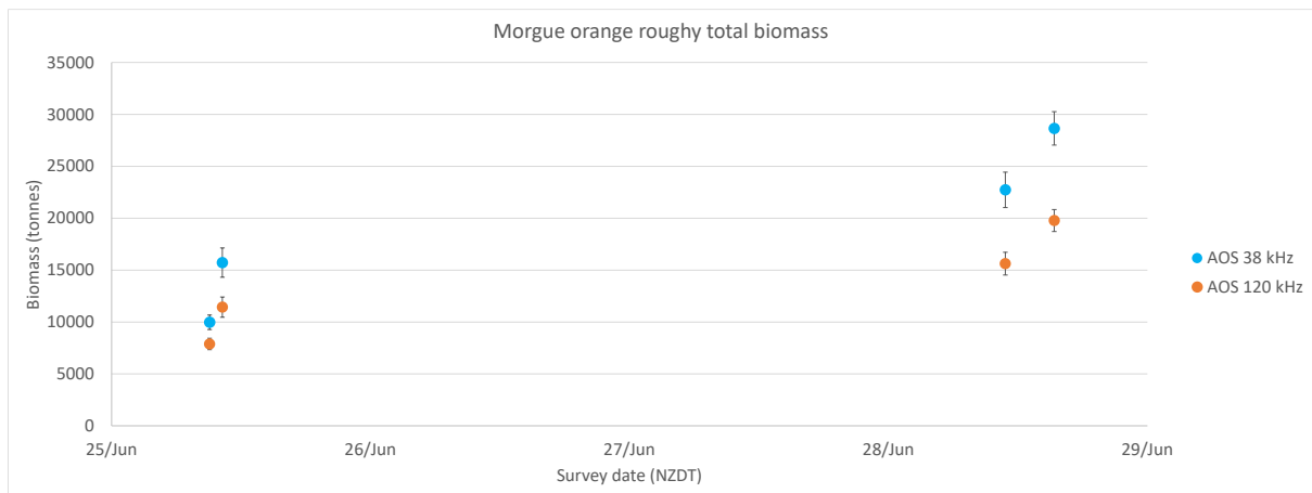
Figure 19. Biomass estimates for AOS surveys of Morgue for 38 and 120 kHz echosounder data. Total biomass including deadzone estimates are shown. Error bars show 1 standard deviation based on survey sampling CV.
