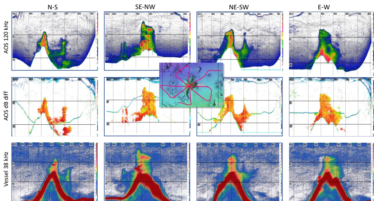
Figure 14: AOS survey at the Morgue. OP39, 28 June 2022 22:33. Top images show the AOS ES60 120 kHz echograms. Lower set of images shows the vessel ES80 38 kHz echograms. Middle set of images shows the subtraction of 120 kHz from 38 kHz backscatter. Orange pixels show backscatter at 120 kHz is \sim twice as high as 38 kHz, indicative of large fish without a gas bladder (e.g. orange roughy). Green pixels occur when backscatter signal is approximately equal on both frequencies indicating large gas bladder species. The map shows star pattern vessel survey track over the top of the Morgue feature.
