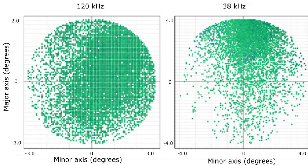
Figure 3: Location of reference target sphere within the acoustic beam for 120 and 38 kHz AOS echosounders for all platform depths.
