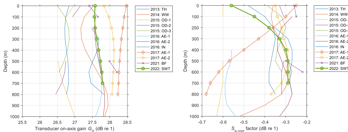
Figure 5. Profiles of gain vs depth (left panel) and S_a correction vs depth (right panel) for 120 kHz AOS transducer.
