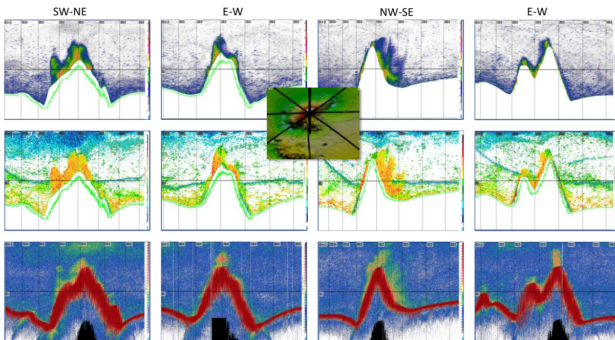
Figure 43: Echograms from second AOS survey of Mt Muck (OP76, 8 July 2022). Top images show AOS 120 kHz echograms. Middle set shows AOS 120 kHz minus 38 kHz where orange pixels are ~ 2 times greater signal at 120 kHz which is indicative of non-gas bladder species – e.g. orange roughy. The bottom set of images shows the vessel ES80 38 kHz echograms.
