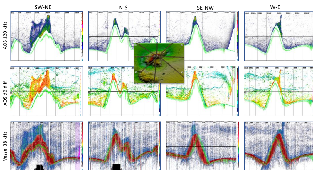
Figure 42: Echograms from first AOS survey of Mt Muck (OP72 6 July 2022). Top images show AOS 120 kHz echograms. Middle set shows AOS 120 kHz minus 38 kHz where orange pixels are ~ 2 times greater signal at 120 kHz which is indicative of non-gas-bladder species – e.g. orange roughy. The bottom set of images shows the vessel ES80 38 kHz echograms.
