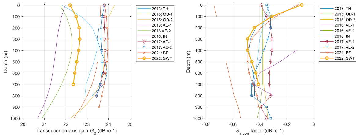
Figure 4. Profiles of gain vs depth (left panel) and S_a correction vs depth (right panel) for 38 kHz AOS transducer.
