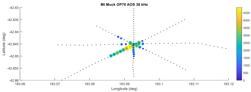
Figure 53. Map of biomass surveys at Mt Muck with circle size indicating backscatter (NASC) value for each echointegration interval. Bubble size is scaled by the largest NASC value for the surveys. Colour bar indicates NASC values.
