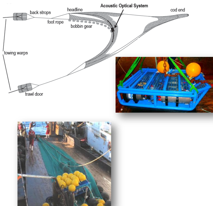
Figure 2. Sealord Acoustic Optical System with conceptual diagram of its attachment to the headline of the demersal trawl net and the system in the trawl net on the aft deck.
