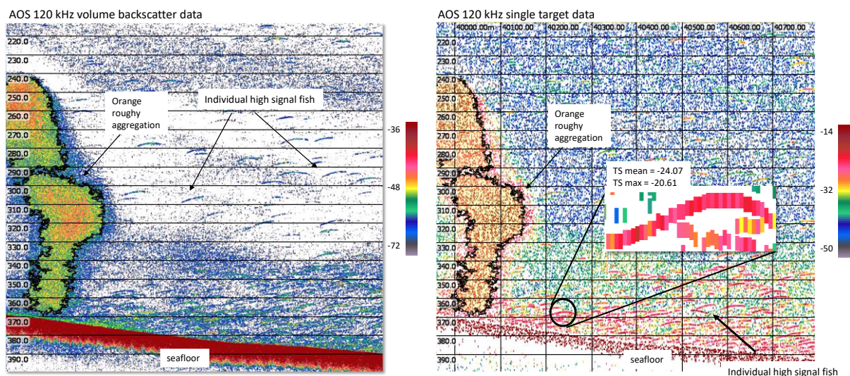
Figure 35: Left image. 120 kHz volume backscatter echogram at Spawn Plume (OP67, 5 July 2022) showing an orange roughly aggregation with backscatter from individual high-signal fish. Right image. Single targets at 120 kHz. The continuous red lines are backscatter from high signal individual fish as they move through the acoustic beam.
