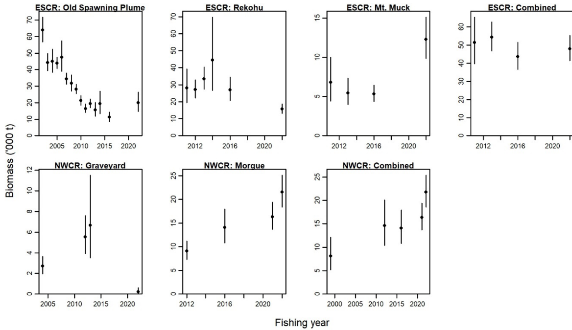
Figure 5: ORH 3B sub-areas and Spawning Stock Biomass estimates from acoustic surveys. ESCR, East and South Chatham Rise; NWCR, Northwest Chatham Rise. Vertical lines indicate 95% CI.
