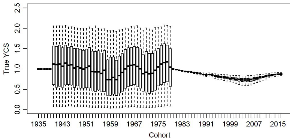
Figure 12: NWCR base, MCMC estimated ‘true’ YCS ( R_t/R_0 ). The box in each year covers 50% of the distribution and the whiskers extend to 95% of the distribution.
