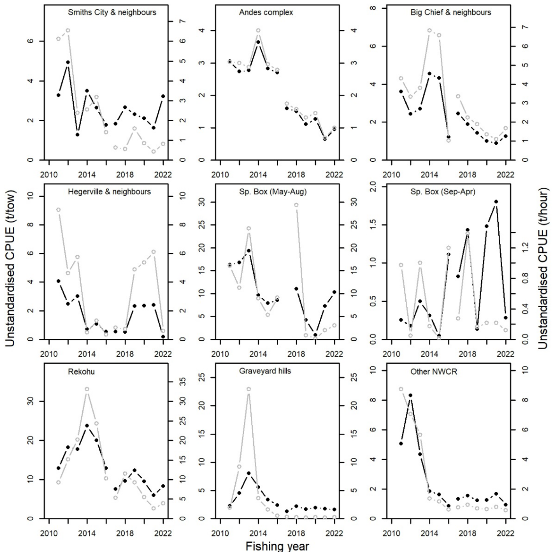
Figure 4: ORH 3B fishery sub-areas and annual unstandardised CPUE for the periods 2009–10 to 2015–16 (period of lower catches and TAC); 2016–17 to 2021–22 (recent years within which fishery characteristics have changed: see text). Black lines and points, t/tow (left y-axis); Grey lines and points, t/hour (right y-axis). Graveyard Hills and Other NWCR are within the NWCR stock, the other sub-areas being within the ECSR.
