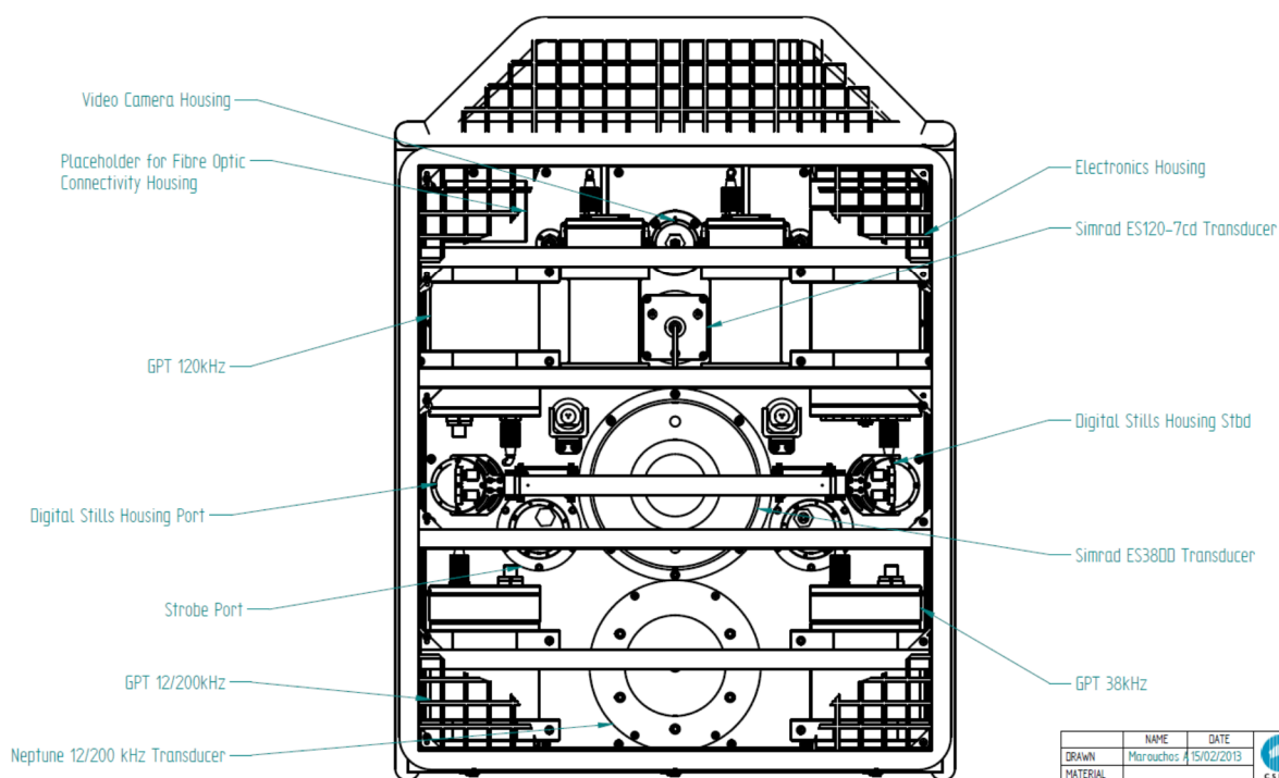
Figure 2. Sealord NZ Acoustic Optical System
