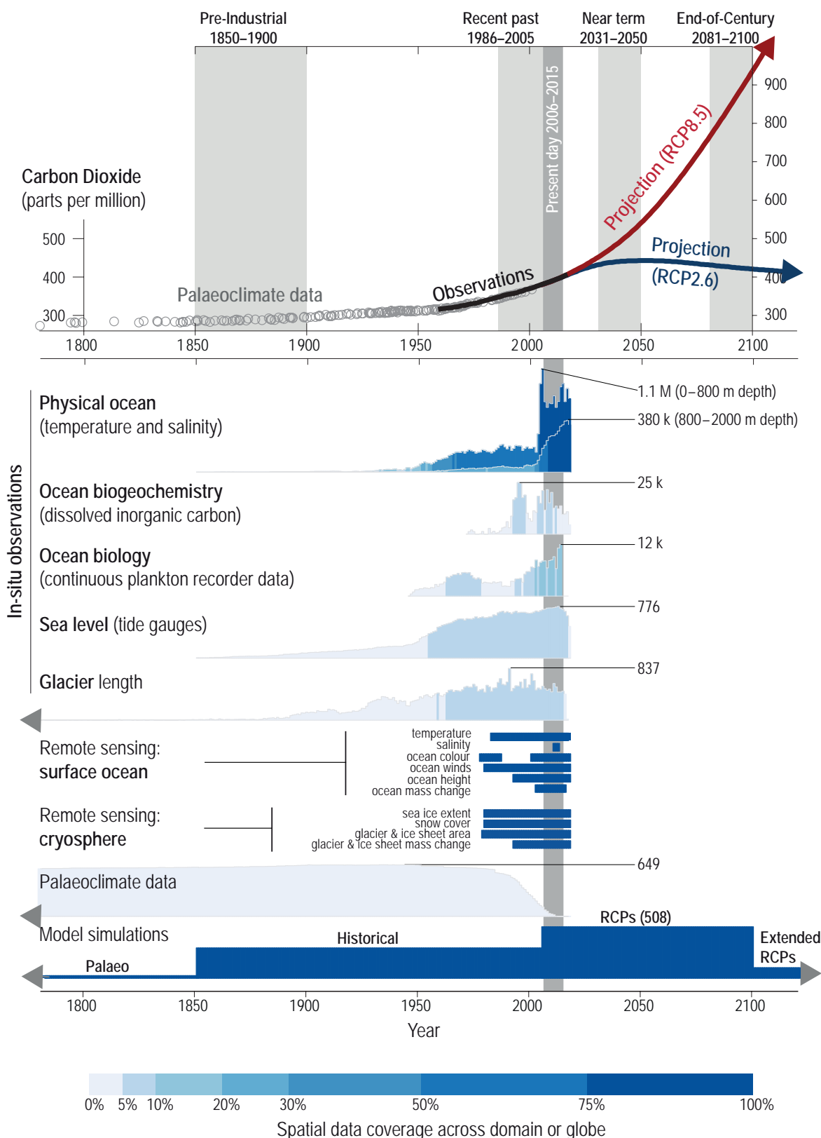
Figure 1.3 | Illustrative examples of the availability of ocean and cryosphere data relative to the major time periods assessed in the Special Report on the Oceans and Cryosphere in a Changing Climate (SROCC). Upper panel; observed (Keeling et al., 1976) and reconstructed (Bereiter et al., 2015) atmospheric CO 2 concentrations, as well as the Representative Concentration Pathways (RCPs) of CO 2 for low (RCP2.6) and high (RCP8.5) future emission scenarios (van Vuuren et al., 2011a; Cross-Chapter Box 1 in Chapter 1). Lower panel; illustrative examples of data availability for the ocean and cryosphere (Section 1.8.1; Taylor et al., 2012; Boyer et al., 2013; Dowell et al., 2013; McQuatters-Gollop et al., 2015; Raup et al., 2015; Olsen et al., 2016; PSMSL, 2016; PAGES2K Consortium, 2017; WGMS, 2017). The amount of data available through time is shown by the heights of the time series for observational data, palaeoclimate data and model simulations, expressed relative to the maximum annual data availability (maximum values given on plot; M = million, k = thousand). Spatial coverage of data across the globe or the relevant domain is shown by colour scale. See SM1.4 for further details.
