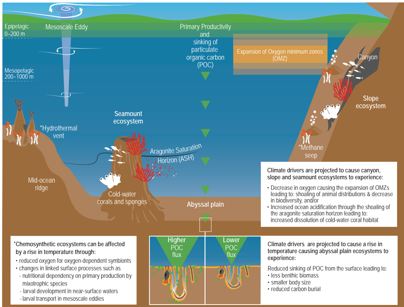
Figure 5.15 | A conceptual diagram illustrating how climate drivers are projected to modify deep sea ecosystems as discussed in Section 5.2.4.
