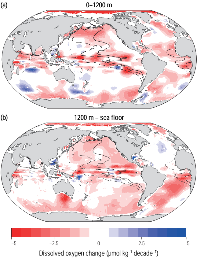
Figure 5.9 | Absolute change in dissolved oxygen (umol kg -1 per decade) between water depths of (a) 0 and 1200 m, and (b) 1200 m and the sea floor over the period 1960–2010. Lines indicate boundaries of OMZs with less than 80 μmol kg -1 oxygen anywhere within the water column (dashed/dotted), less than 40 μmol kg -1 (dashed) and less than 20 μmol kg -1 (solid). Redrawn from Oschlies et al. (2018).
