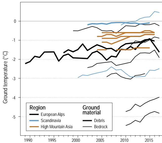
Figure 2.5 | Mean annual ground temperature from boreholes in debris and bedrock in the European Alps, Scandinavia and High Mountain Asia. Temperatures differ between locations and warming trends can be interspersed by short periods of cooling. One location shows degrading of permafrost. Overall, the number of observed boreholes is small and most records are short. The depth of measurements is approximately 10 m, and years without sufficient data are omitted (Noetzli et al., 2018).
