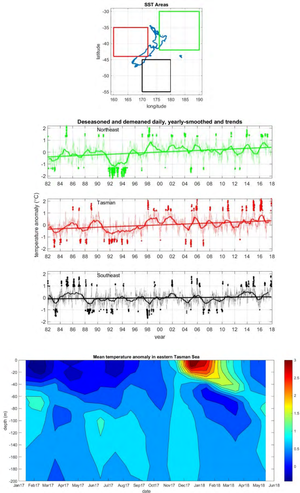
Figure 12.10: Marine heat waves. The top panel shows three regions chosen to represent different regimes. The middle panel shows the mean deseasoned satellite SST values for these regions, at daily and annually-smoothed resolutions. The linear trends are also shown. Values more than two standard deviations from the mean are shown in bold. (Modified from Sutton & Bowen 2019). The bottom panel shows the mean temperature anomaly in the eastern Tasman Sea through the summer of 2017–2018. (Modified from Salinger et al. 2018)
