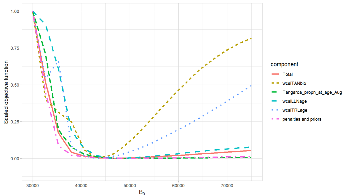
Figure 5: Likelihood profiles of the base case model for the virgin spawning stock biomass parameter ( B_0 ) for each likelihood component: likelihood profile of all the components (Total); survey biomass estimates (wcsiTANbio); survey proportions at age (Tangaroa_propn_at_age_Aug); age distributions in catches by the longline fishery (wcsiLLNage); age distributions in catches by the trawl fishery (wcsiTRLage); and model penalties and priors (penalties and priors).
