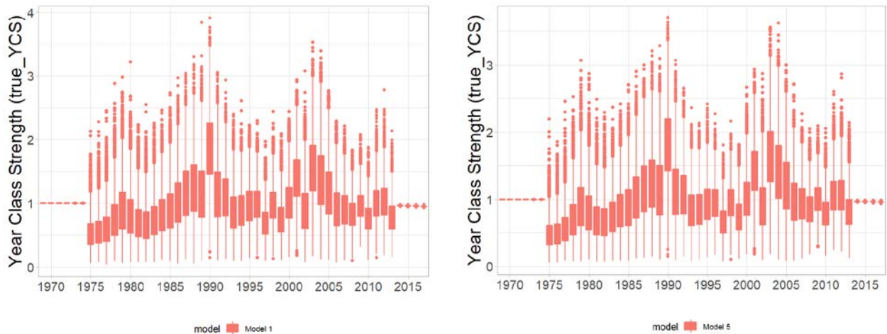
Figure 11: Estimated recruitment trends and variability by model 1 (left hand side) and model 5 (right hand side).
