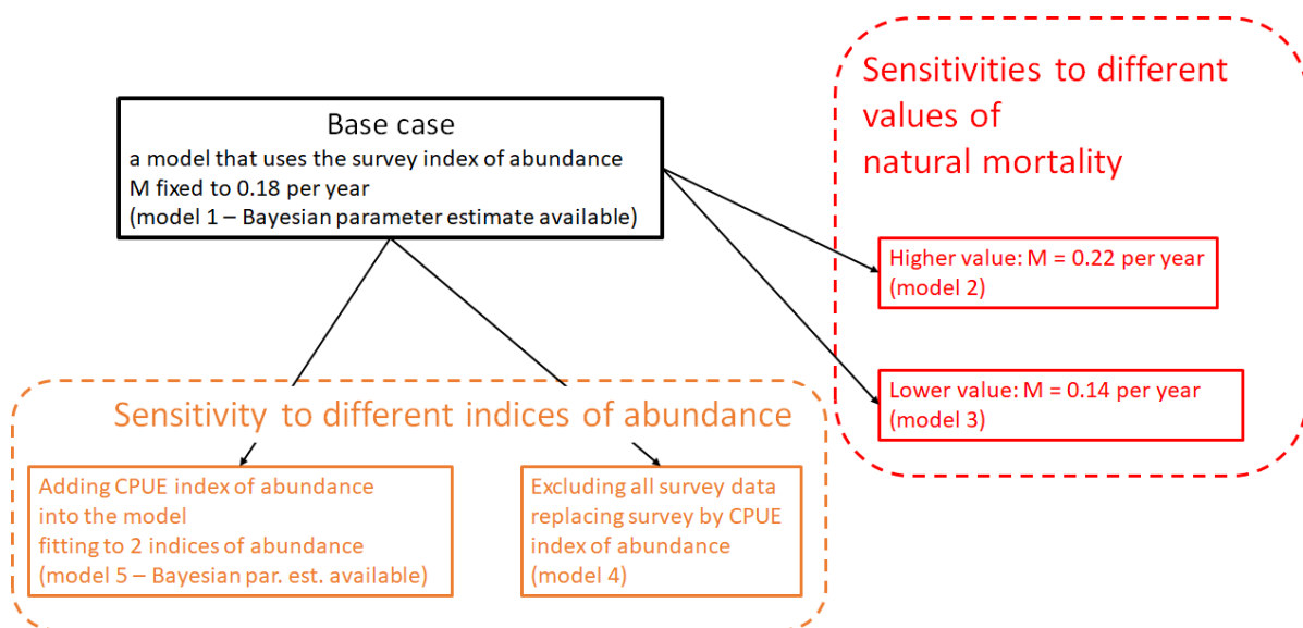
Figure 4: Relationship between the base case model and 4 alternative models. ‘Bayesian par.est.’ is Bayesian parameter estimate.
