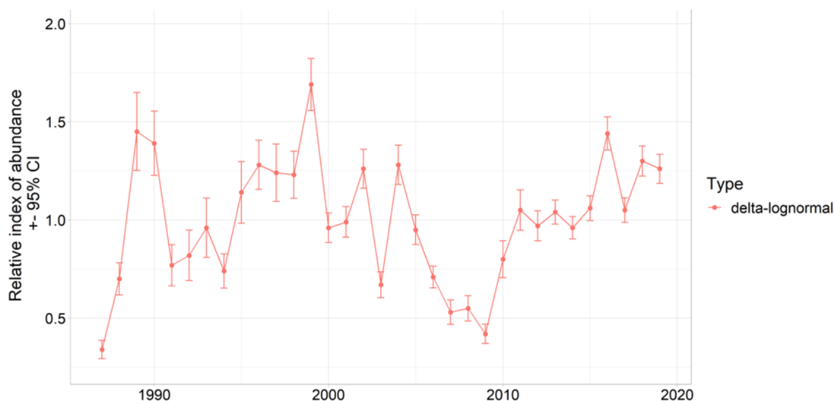
Figure 3: The CPUE index of abundance obtained by standardising the commercial trawl fishery catch and effort data (x-axis labelled as fishing year-ending).
