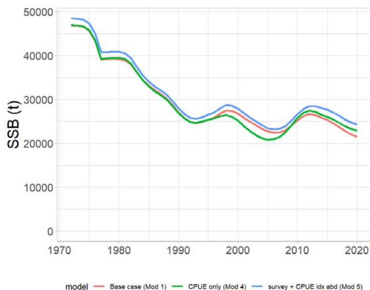
Figure 8: Trends in Spawning Stock Biomass ( SSB ) estimated by 3 models to assess the sensitivity of the stock assessment to using different indices of abundance.
