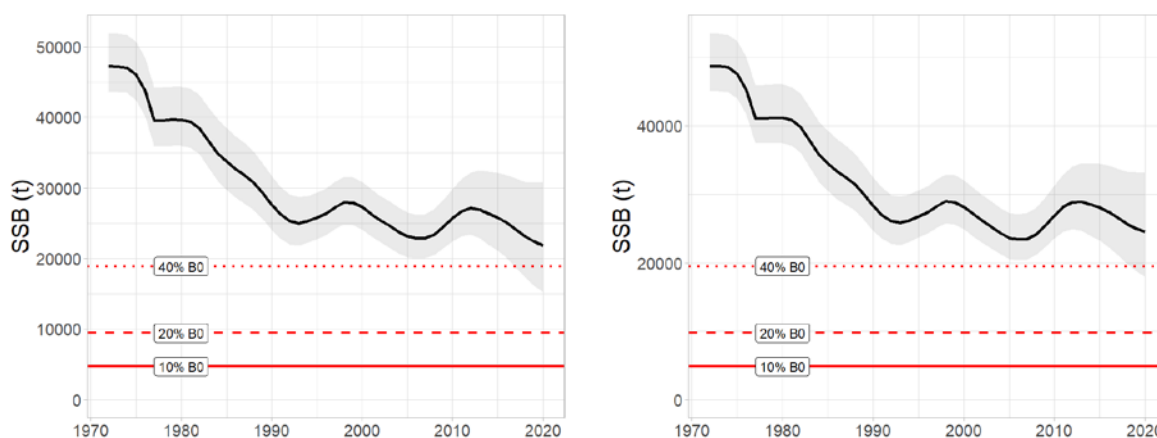
Figure 10: Estimated trends in Spawning Stock Biomass ( SSB , in tonnes) using the base case model (left hand side) and model 5 (right hand side). The black line shows the median and the grey area the boundaries of the 95% confidence intervals. The horizontal red lines give the management reference points.
