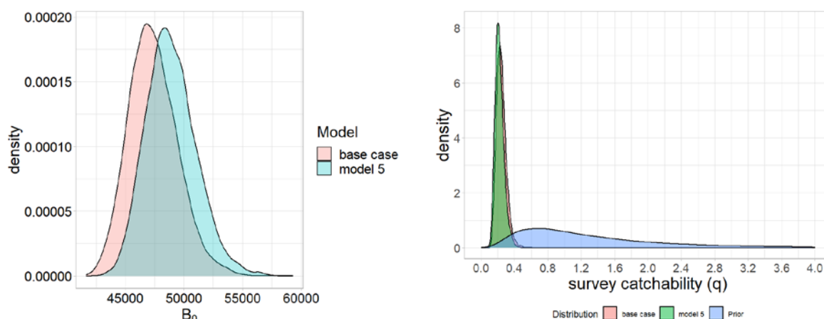
Figure 9: Comparison of the posterior distributions of virgin spawning stock biomass ( B_0 , left hand side) between the base case model and model 5. Comparison of the posterior distribution of survey catchability between the base case and model 5 and its prior distribution.
