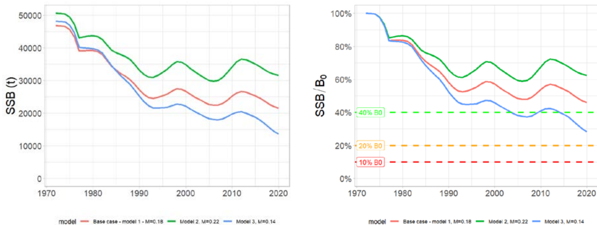
Figure 7: Trends in Spawning Stock Biomass ( SSB ) estimates by the base case model and model 2 and 3: (left hand side) estimates of absolute SSB ; (right hand side) estimate of SSB relative to virgin spawning stock biomass ( B_0 ).
