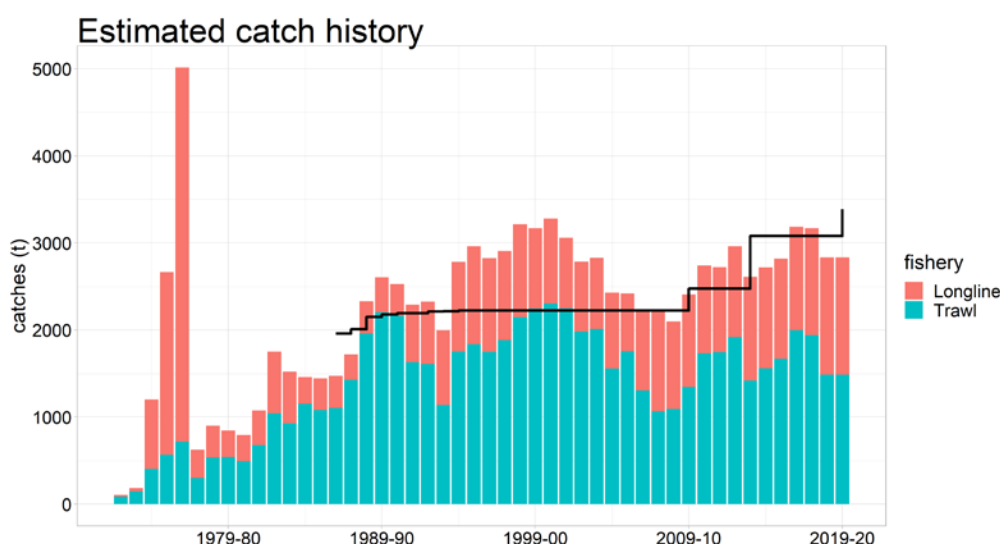
Figure 2: Time series of ling catches in LIN 7WC by fishery. The black line indicates the TACC.
