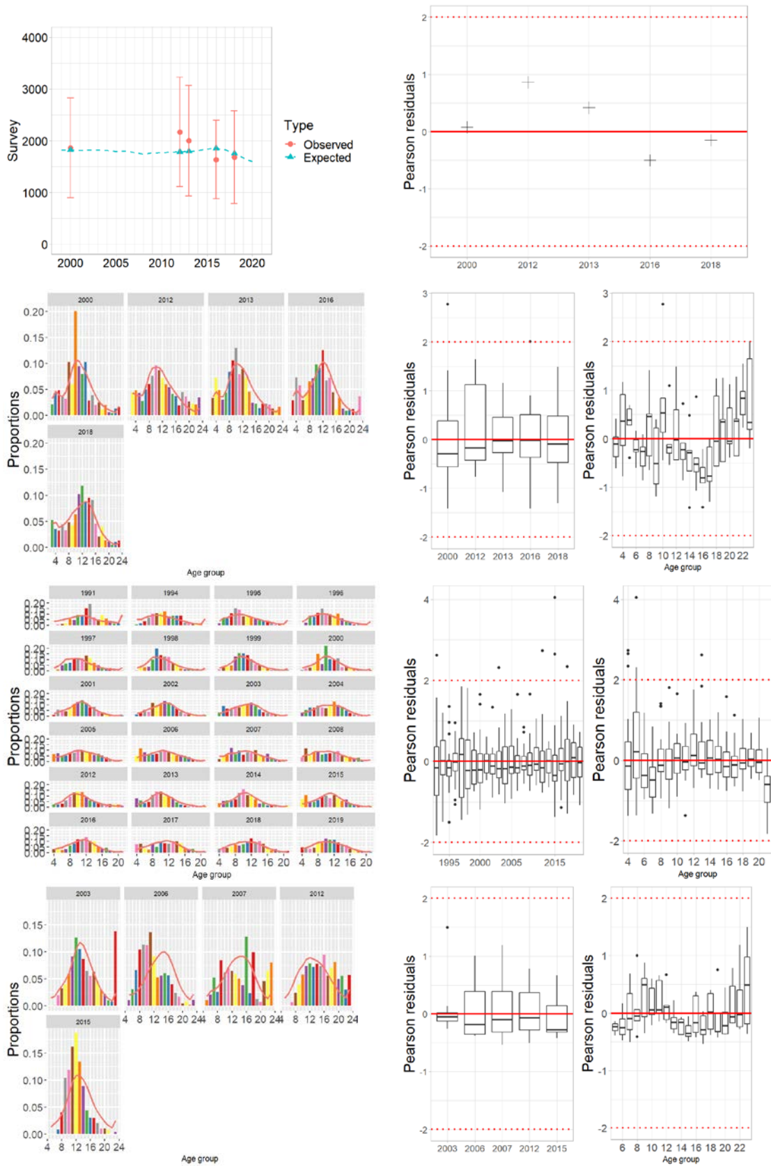
Figure 6: Diagnostics of the fit of the base case model: the left hand side column shows the data overlaid with the model and the right hand side shows the Pearson residuals for each dataset. Row 1 presents the fit to the index of abundance from the scientific surveys; row 2, the fit to the age composition in the scientific surveys; row 3, the fit to the age composition in the trawl fishery catches and row 4, the fit to the age composition in the catch from the long line fishery.
