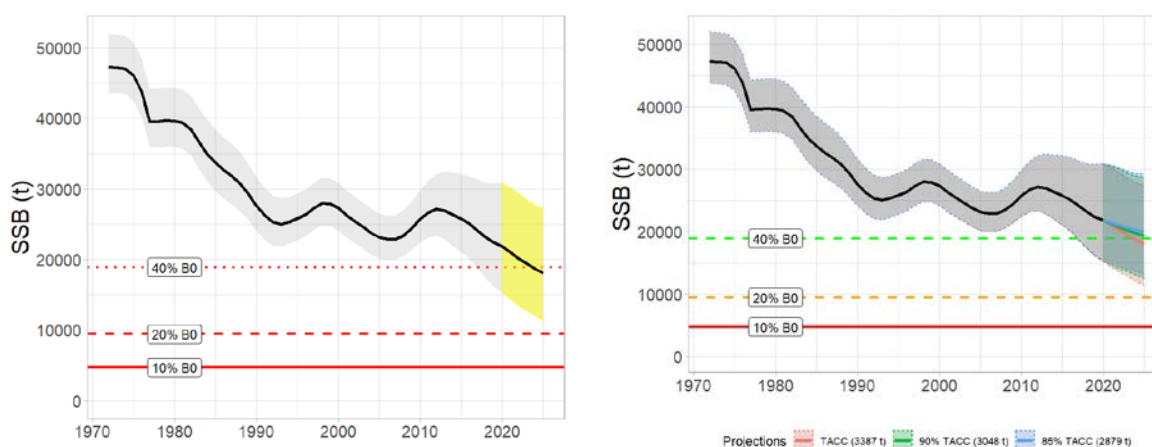
Figure 13: Projected trends in Spawning Stock Biomass ( SSB , in tonnes) to 2025 using future annual catches equal to the TACC in 2020 and the last 10 years of recruitment estimates (left hand side). The right-hand side compares trajectories of ling SSB with future catches set at 85, 90, and 100% of the TACC in 2020.
