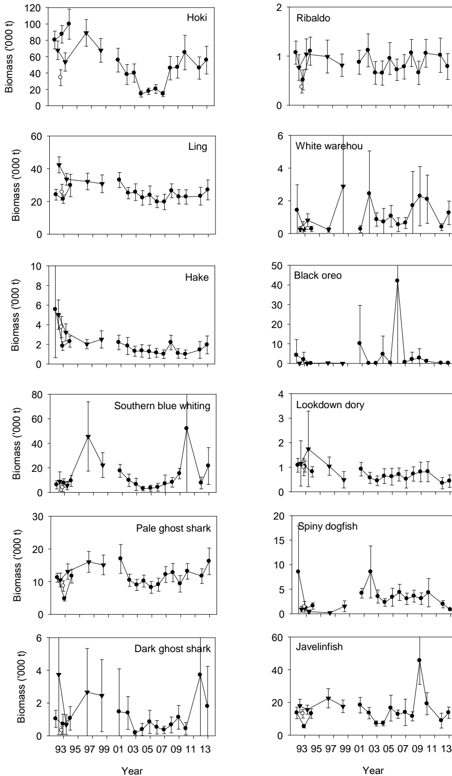
Figure 3: Trends in biomass ( \pm 2 standard errors) of key species in the core 300–800 m strata in all Sub-Antarctic trawl surveys from Tangaroa. Solid circles show the summer time series and solid triangles the autumn time series. The open circle shows biomass from a survey of the same area in September–October 1992.
