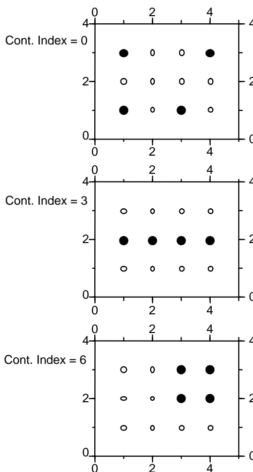
Figure 10.4.3.4.2.1 Samples of contagion index.
