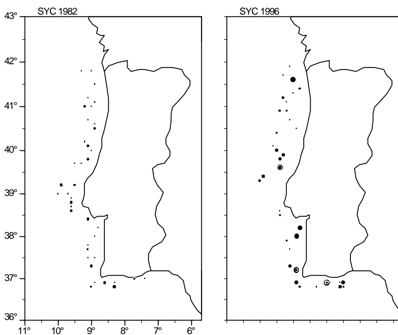
Figure 10.4.3.4.1 Sample data from the Portuguese survey series. The figure contains the aggregated biomass for Scyliorhinus canicula 1982 and 1996. Larger circles reflect higher abundance.
