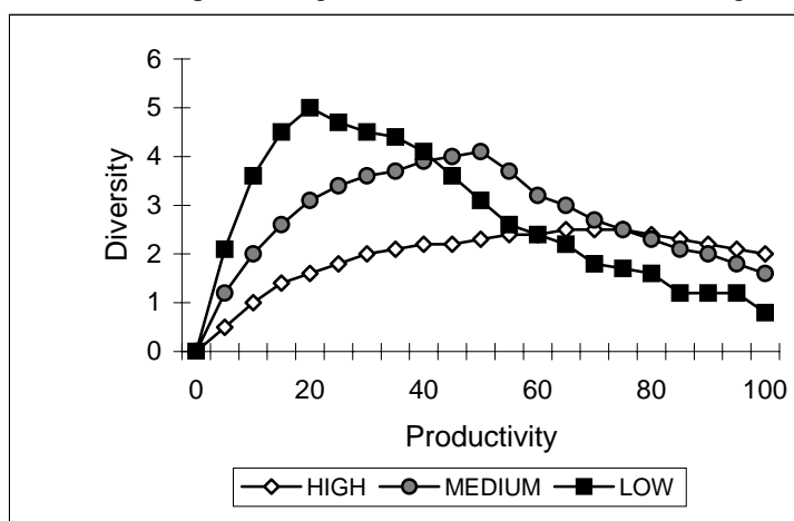
Figure 9.3.1.3 Effect of disturbance on the mean diversity and standard deviation estimated over the full productivity range. Low, medium, and high disturbance ranges shown on Figures 9.3.1.2 and 9.3.1.4 correspond to regions labelled low, medium, and high in Figure 9.3.1.1.
