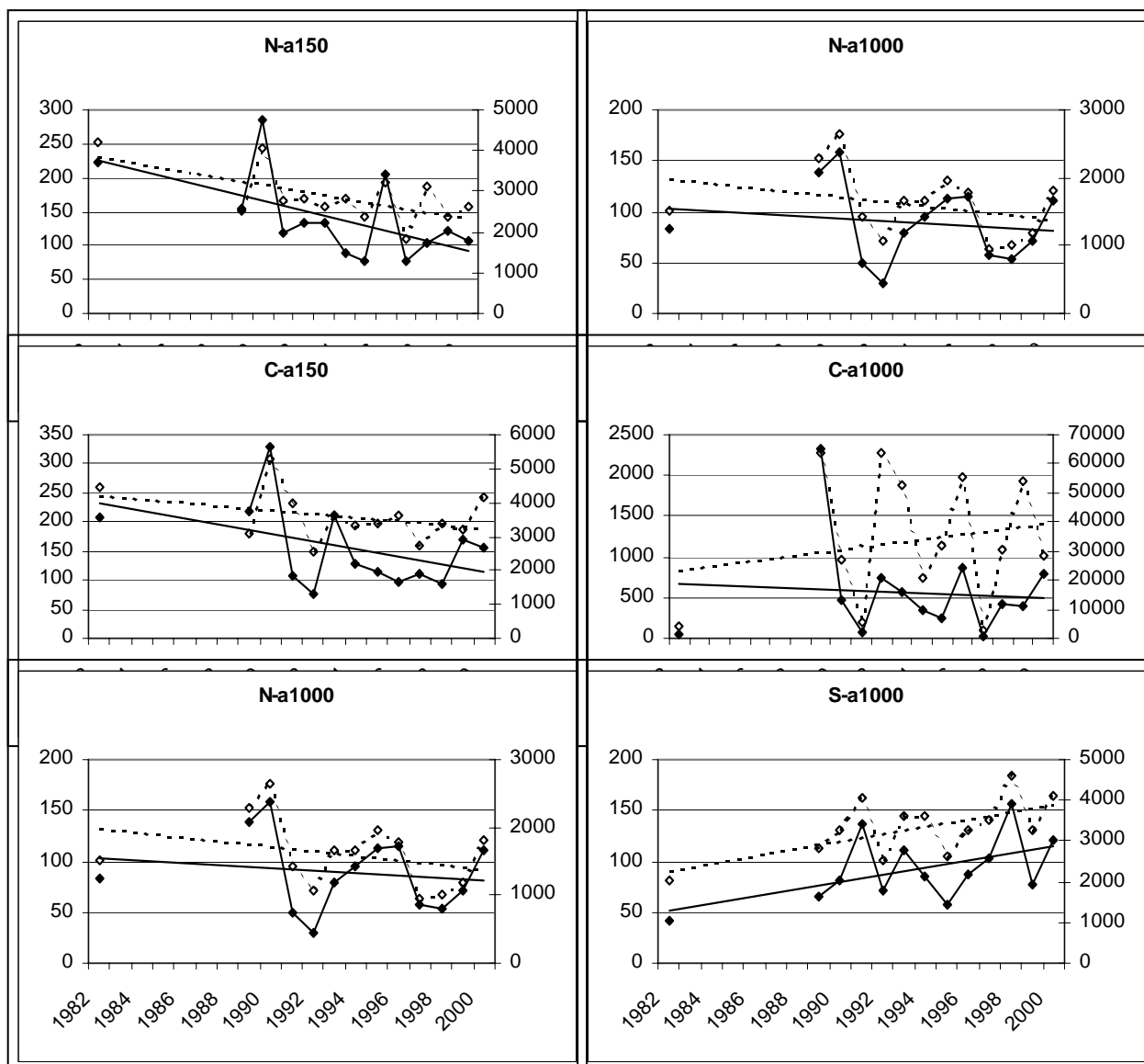
Figure 10.4.3.3.1 Plots of weighted averages of L_{\max} and trophic level for 6 groups (N=North, C=Centre, S=South; a150=1–150 m, a1000=151 to 1000 m). Solid lines for L_{\max} , dashed lines for trophic level.
