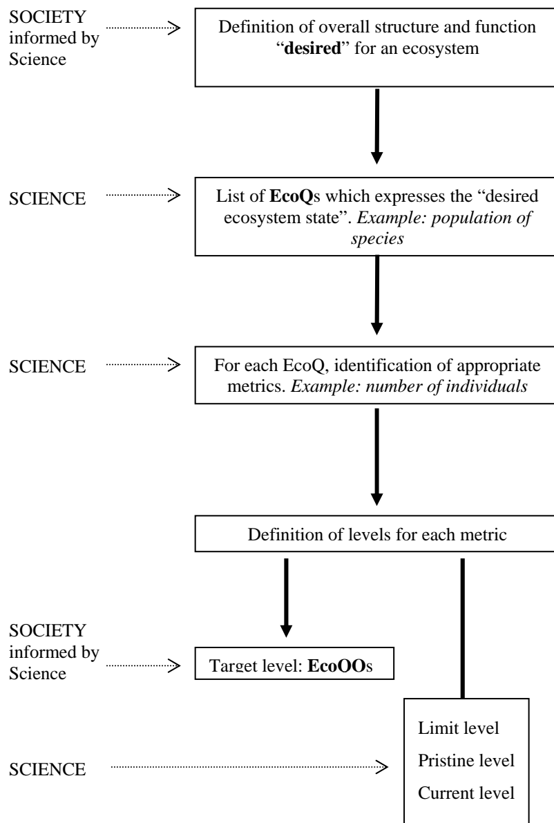
Figure 3.1.1 Conceptual framework for the methodology of describing EcoQ and setting EcoQOs (from Lanter et al. , 1999).
