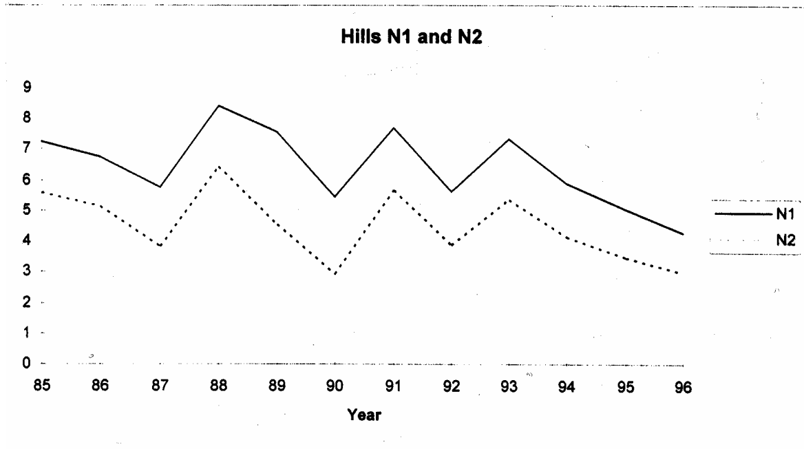
Figure 8.2.2.2.2 Hills N1 and N2 calculated from a series of 12 years of the Norwegian bottom trawl survey in the Barents Sea.
