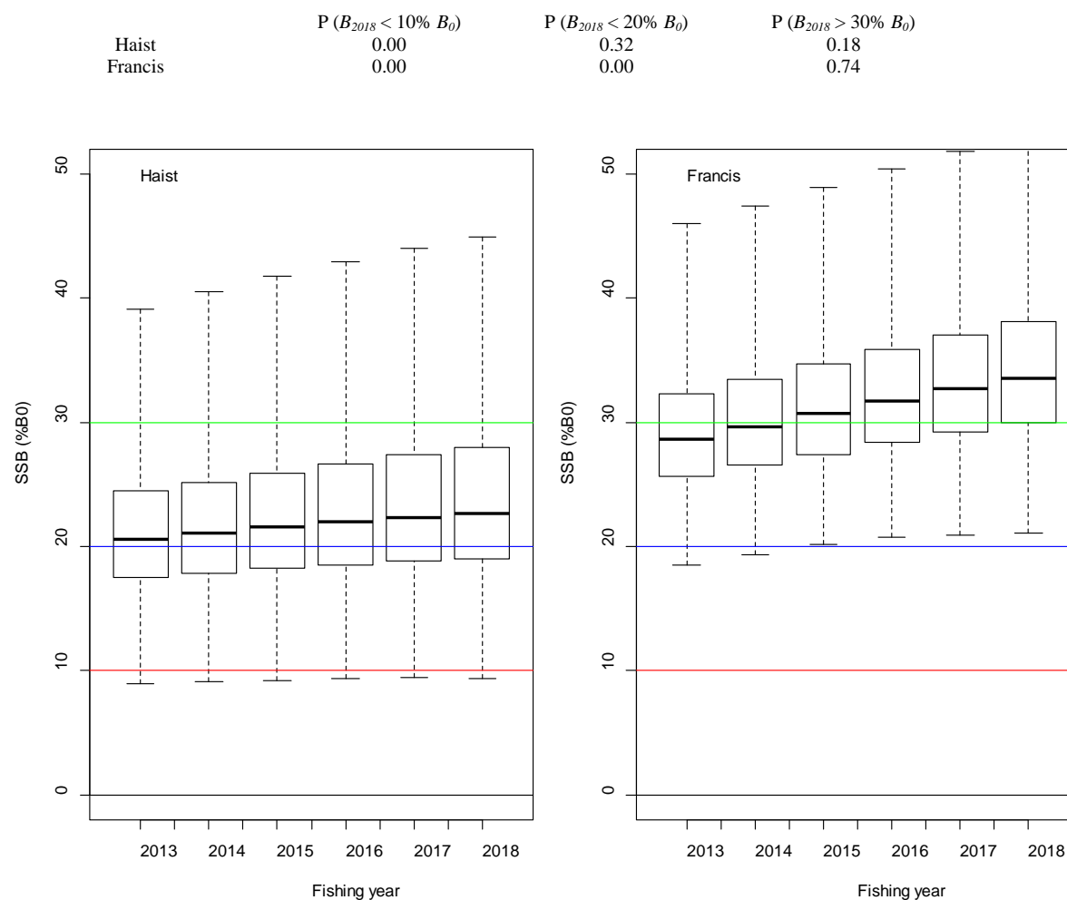
Figure 18: MCMC projection results at the current catch limit (930 t) assuming a 66-34% split between north and south catches and a 5% over-run. The box contains 50% of the distribution and the whiskers extend over the full range.
