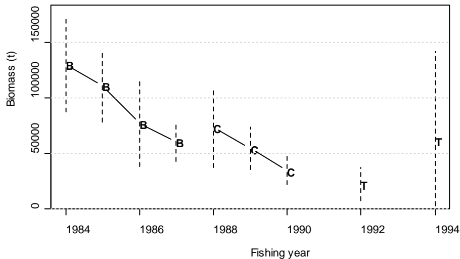
Figure 5: The Spawning Box trawl survey biomass index (assuming a catchability of 1 for each vessel), with 95% confidence intervals shown as vertical bars. Vessels indicated as B, FV Otago Buccaneer ; C, FV Cordella ; T, RV Tangaroa .
