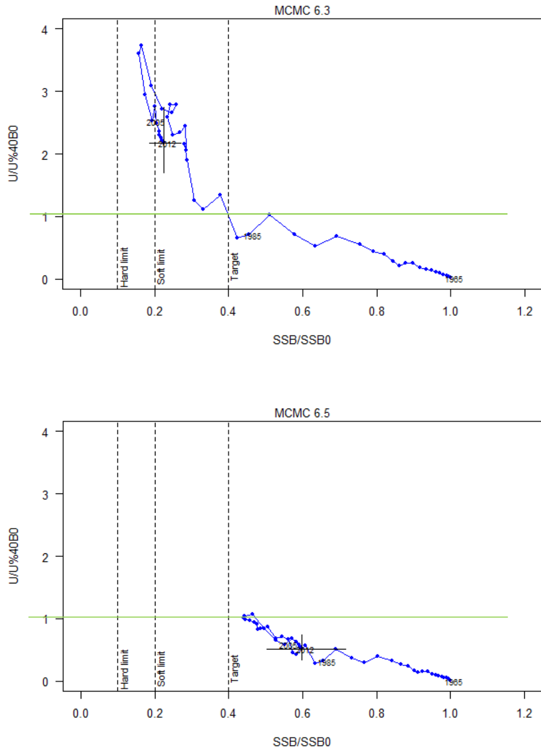
Figure 1 [Continued]: Trajectory of exploitation rate as a ratio of U_{40B0} and spawning stock biomass as a ratio of B_0 from the start of assessment period 1965 to 2012 for MCMC 5.2 (base case), 5.5 (no early CPUE), 6.3 (fast growth), and 6.5 (slow growth). The vertical lines at 10%, 20%, 40% B_0 represent the hard limit, the soft limit, and the target respectively. U_{40B0} is the exploitation rate at which the spawning stock biomass would stabilise at 40% B_0 over the long term. Each point on trajectory represents the estimated annual stock status: the value on x axis is the mid-season spawning stock biomass (as a ratio of B_0 ) and the value on the y axis is the corresponding exploitation rate (as a ratio U_{40B0} ) for that year. For all the models, the trajectory started in year 1965 when the SSB is close to B_0 and the exploitation rate is close to 0. The Estimates are based on MCMC median and the 2012 90% CI is shown by the cross line.
