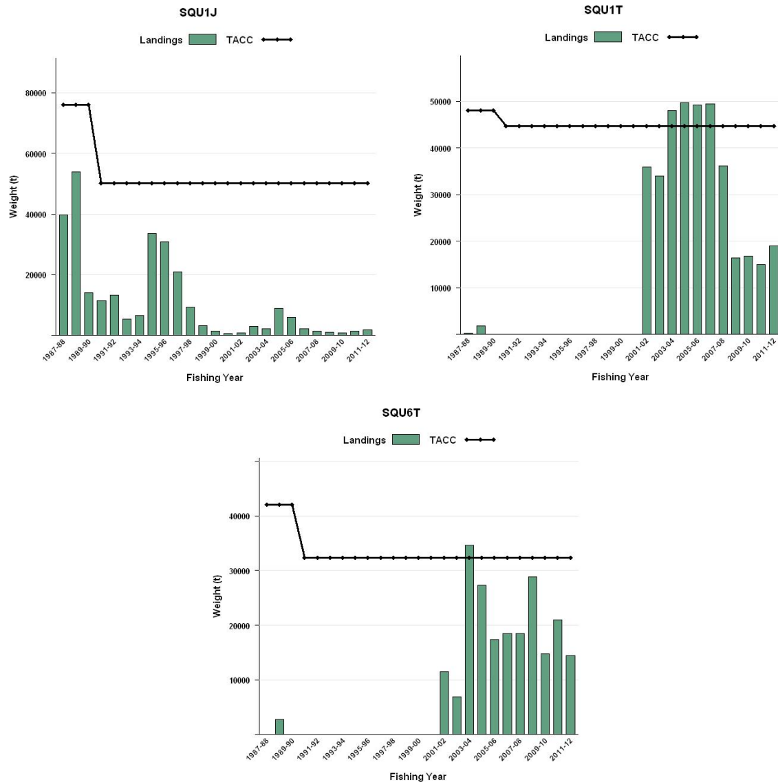
Figure 1: Historical landings and TACC for the three main SQU stocks. Left to right: SQU1J (All Waters Except 10T and 6T, Jigging), SQU1T (All Waters Except 10T and 6T, All Other Methods) and SQU6T (Southern Islands, All Methods). Note that these figures do not show data prior to entry into the QMS.
