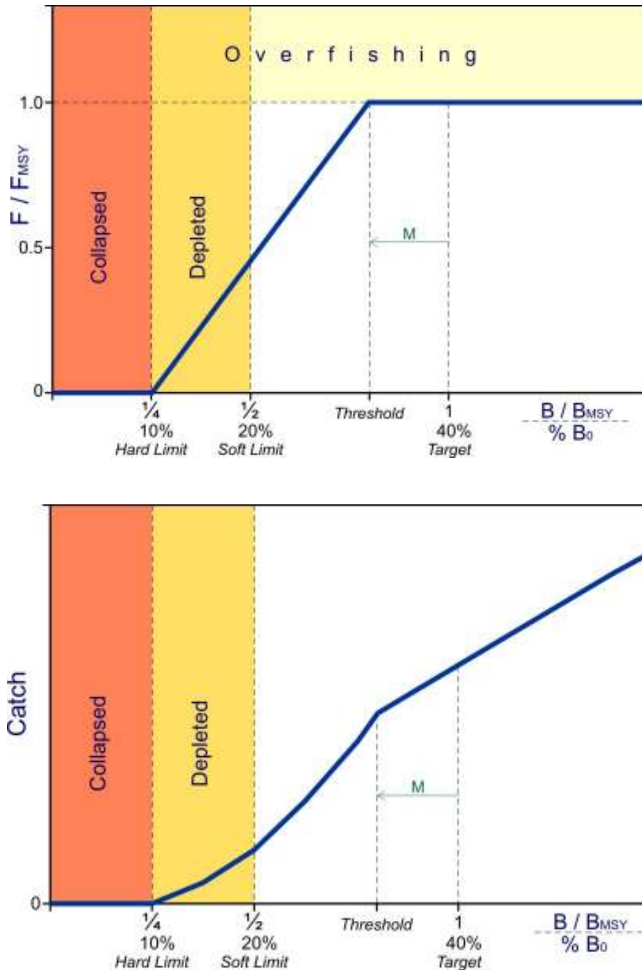
Figure 2. Illustrative example of a harvest strategy control rule that would be in conformance with the Harvest Strategy Standard. The top graph illustrates the control rule applicable for a fishing mortality based strategy, while the bottom graph translates the fishing mortality axis into related catch levels. M is natural mortality.
