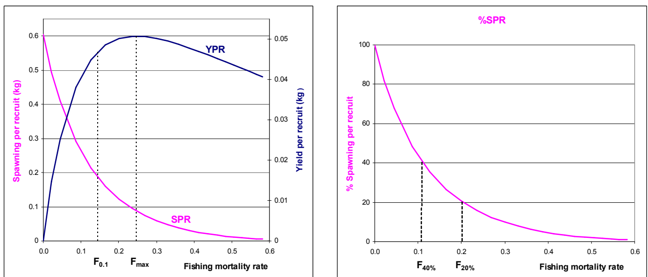
Figure A1: Yield per recruit and spawning biomass per recruit curves.
