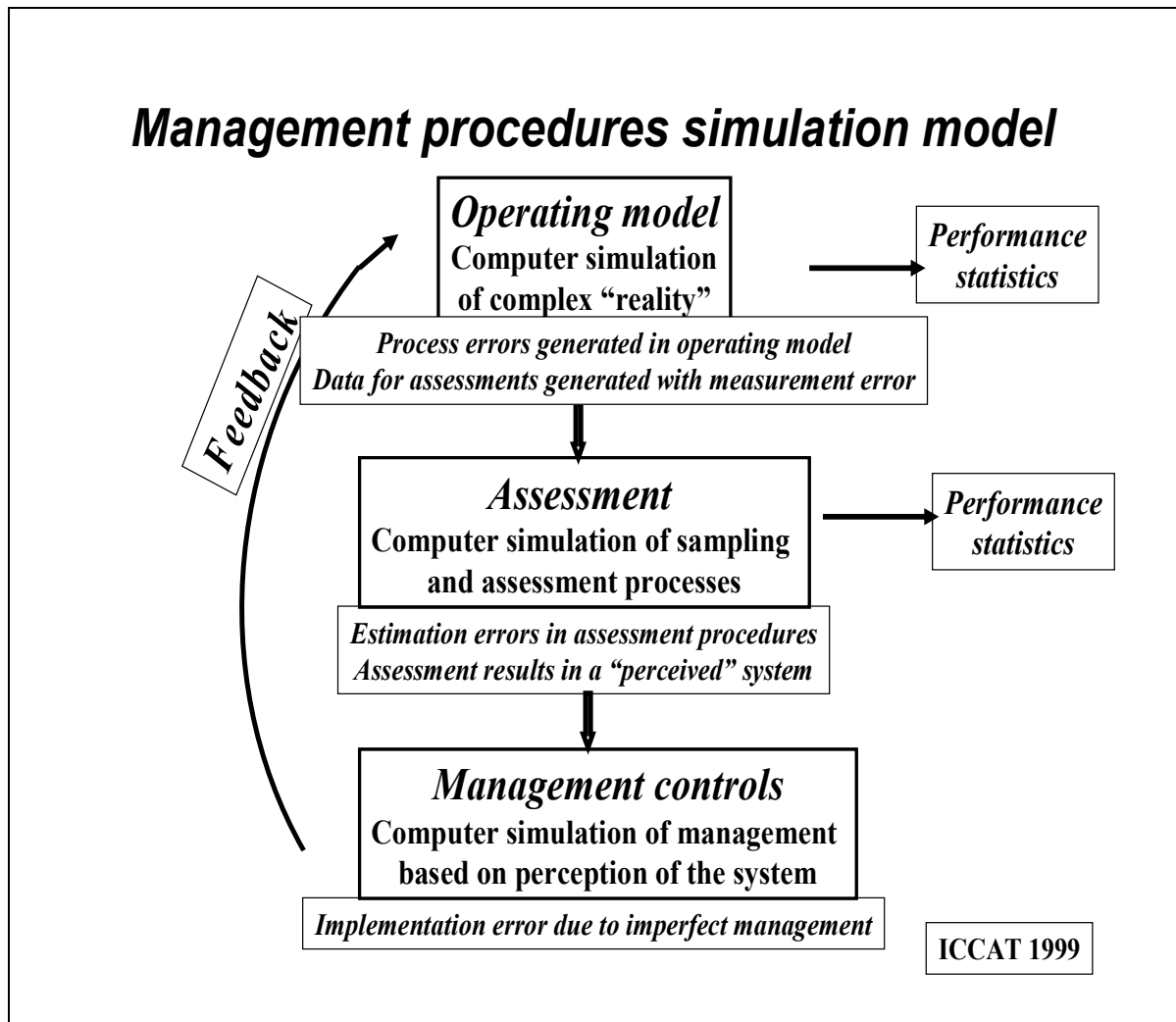
Figure A4: Example of MSE / OMP (ICCAT 1999)
