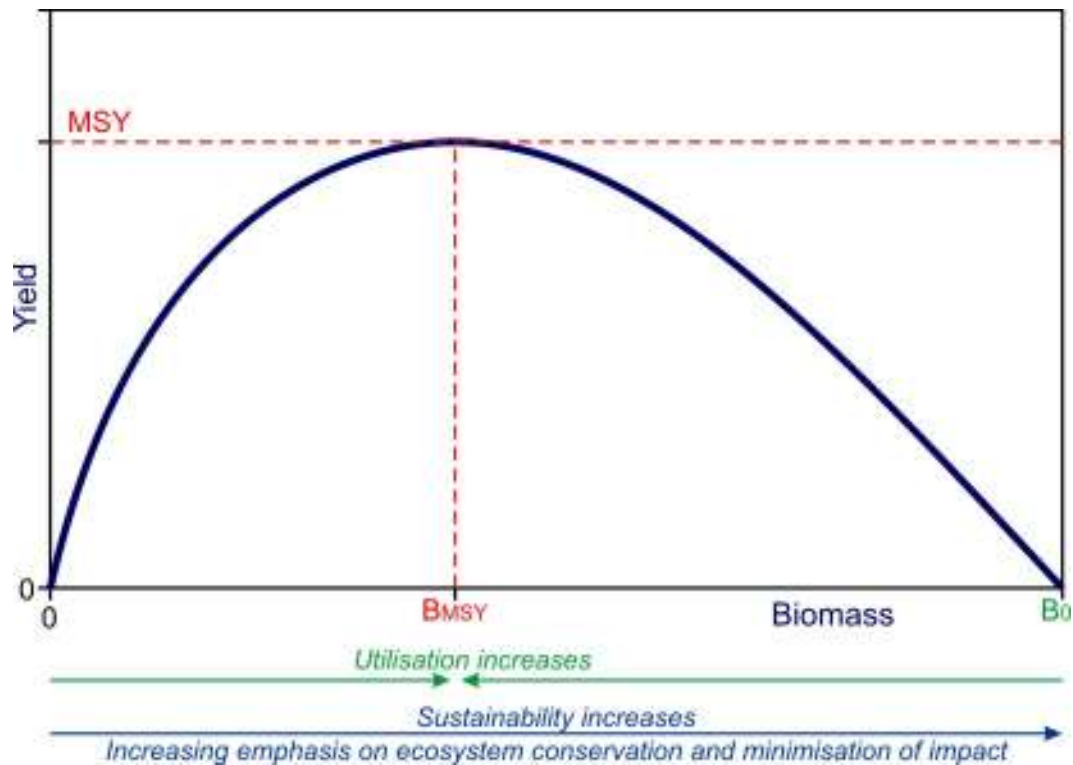
Figure 1. The long-term average (equilibrium) implications of providing for utilisation while ensuring sustainability in an MSY context. Arrows underneath the figure show that utilisation and sustainability considerations act in the same direction when biomass is below B_{MSY} , but in opposite directions when it is above.
