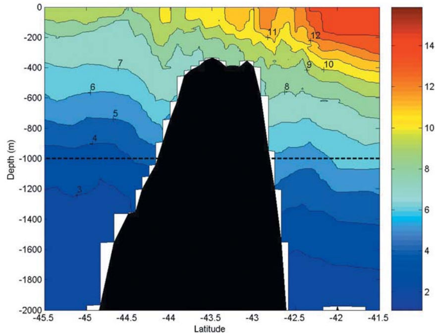
Figure 7. Temperature ( ^{\circ}\text{C} ) across Chatham Rise at 178^{\circ}30\text{E} as measured in October 2000. The horizontal dashed line locates the 1000-m depth for reference.
