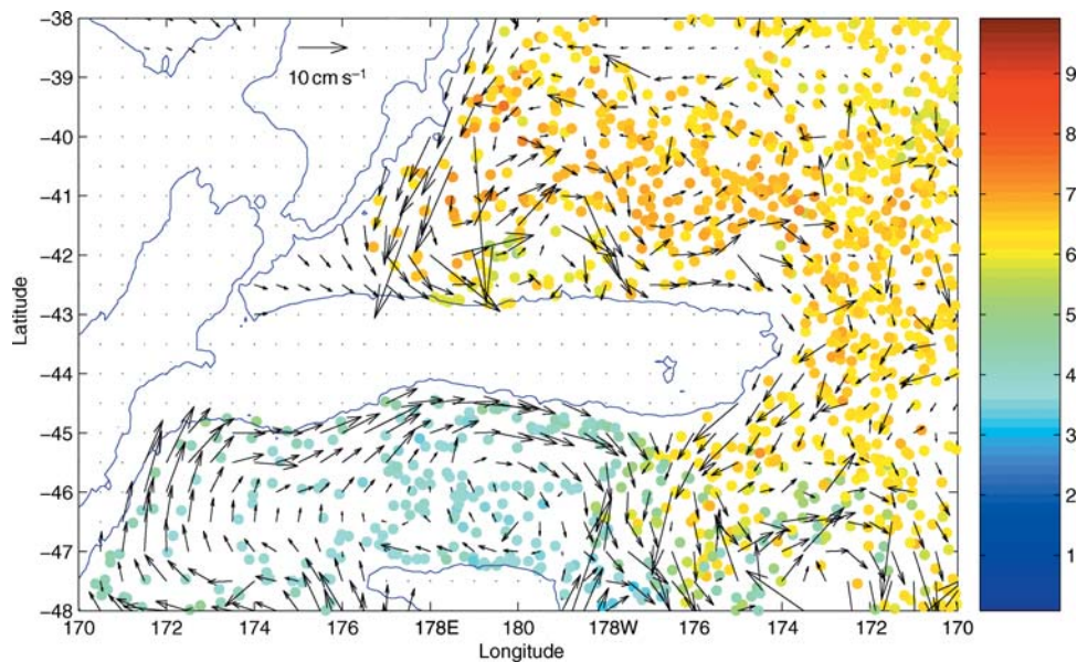
Figure 9. Temperature measured at 900 m from Argo float profiles, with estimates of the velocity at 900 m overlaid. The velocity vectors have been averaged in 0.5^\circ latitude and longitude bins.
