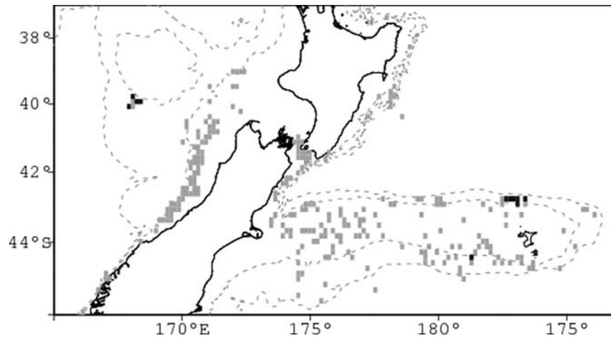
Figure 6. Occurrence of orange roughy in midwater trawls in the 22–27 and 28+ cm SL classes. Only orange roughy of 28 cm SL and over were caught on Mt Kiso (south Chatham Rise). Grey-shaded areas were sampled, and black-shaded areas show where orange roughy were caught. The broken lines indicate the 750- and 1500-m isobaths.
