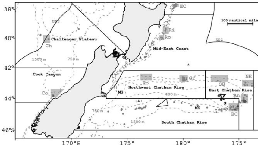
Figure 1. The study area, with the stock boundaries shown as solid lines. The locations of known spawning areas are shown shaded, and are labelled: Ri, Ritchie Bank; Ro, Rockgarden; Ho, the Hole; Gr, Graveyard complex; SB, Spawning Box; NE, Northeast Hills; An, Andes complex and neighbours; BC, Big Chief and neighbours; Ch, Challenger Plateau; Co, Cook Canyon; EC, East Cape hills. Other labels are: MG, Mernoo Gap; MK, Mt. Kiso; triangles, knolls and seamounts (>500 m elevation); dots, hills (<500 m elevation); EEZ, Exclusive Economic Zone boundary. Only the seamounts, hills, and knolls with a summit depth of <1500 m are shown.
