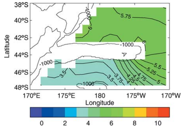
Figure 10. WOA 2005 temperature ( ^\circ\text{C} ) at 1000 m for the area east of New Zealand. Temperature contours are plotted every 0.25^\circ\text{C} , with the 1000-m isobath labelled.
