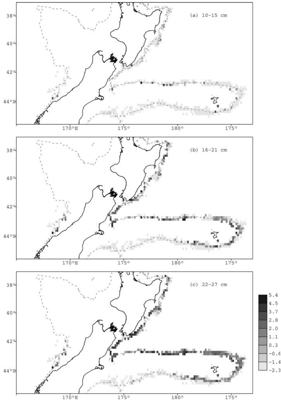
Figure 5. Density of orange roughy by length class from catches in the rough-bottom trawl. The broken line indicates the 1000-m isobath.
