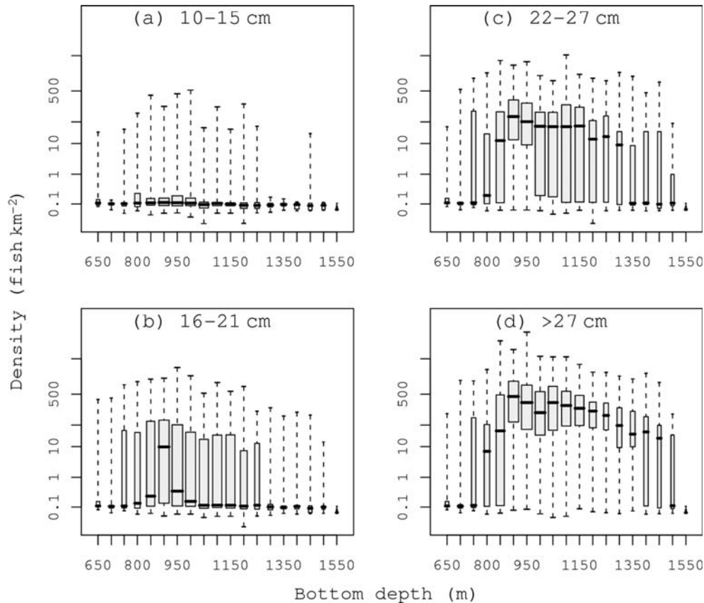
Figure 4. Density of orange roughy (log scale) in rough-bottom net tows by 50-m depth bin and length class. The box limits extend from the lower to the upper quartile, with the solid line indicating the median, and the whiskers extend to the most extreme values. Bar width is proportion to the square root of the number of tows ( n = 3\text{--}332 ).
