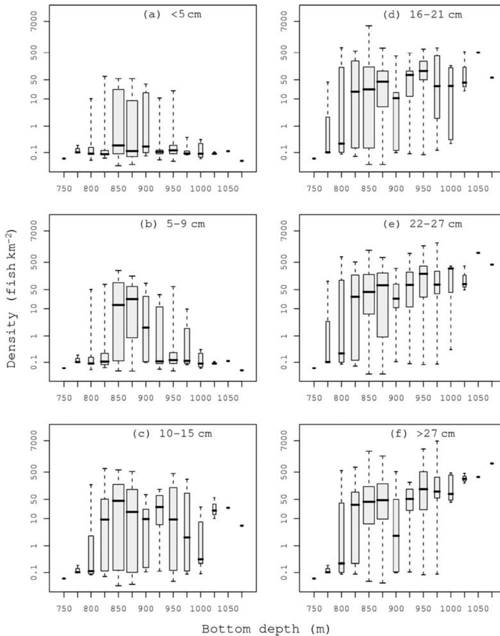
Figure 3. Density of orange roughy (log scale) in prawn-trawl surveys by 25-m depth bin and length class. The box limits extend from the lower to the upper quartile, with the solid line indicating the median, and the whiskers extend to the most extreme values. Bar width is in proportion to the square root of the number of tows ( n=1-37 ).
