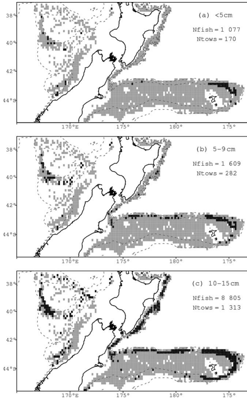
Figure 2. Occurrence of orange roughy in bottom trawls by length class. Grey-shaded areas were sampled, and black-shaded areas show where orange roughy were caught. The broken lines indicate the 750- and 1500-m isobaths. Nfish, number of orange roughy caught; Ntows, number of tows in which orange roughy were caught (out of the total of 12 541 tows) ( Continued ).
