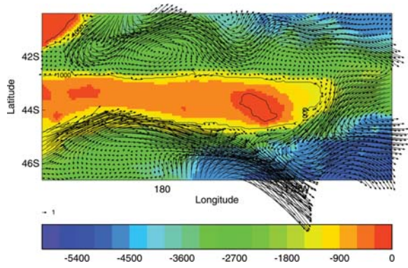
Figure 8. Horizontal velocity vectors at 990 m from the climatological ocean model plotted on top of the model bathymetry from 0 to 6000 m, with the 1000-m isobath labelled. The reference vector indicates a flow speed of 1 \text{ cm s}^{-1} . Model solution has a horizontal resolution of 1/12^\circ of latitude and longitude, and every second horizontal point is plotted for clarity.
