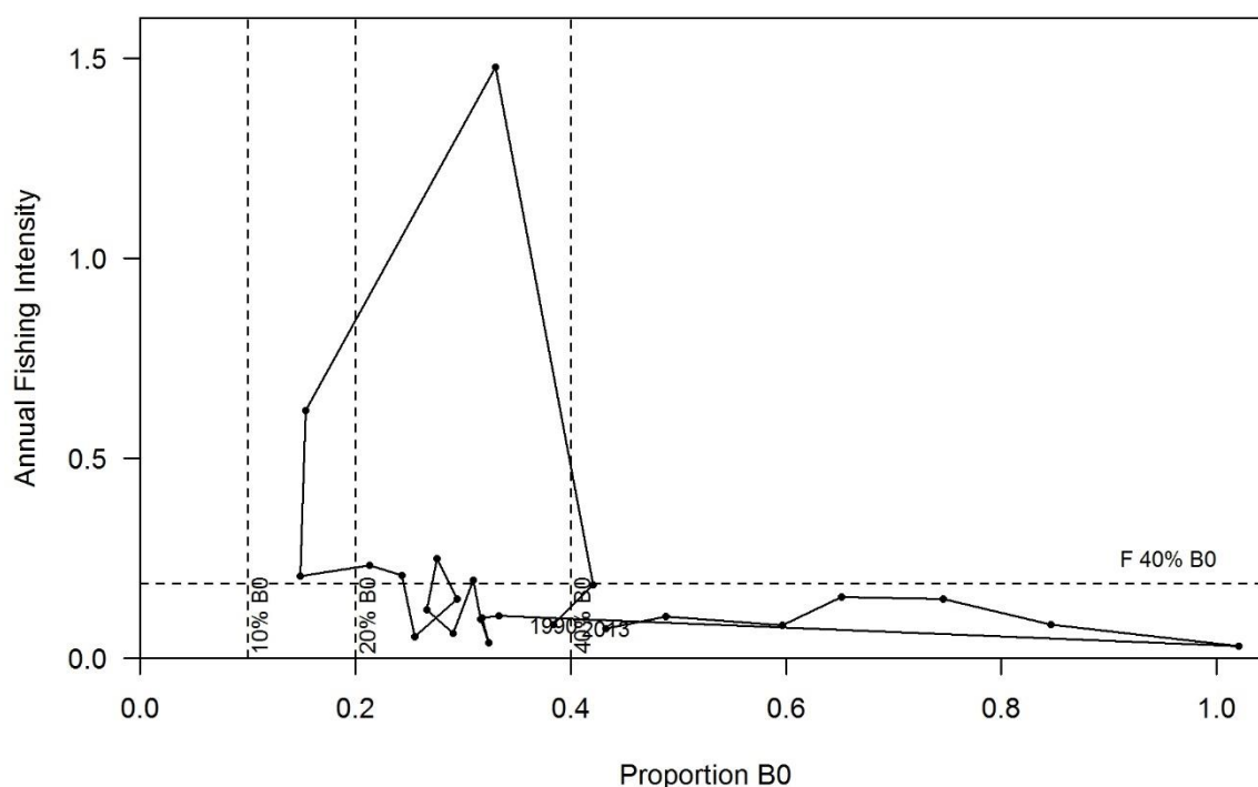
Trajectory over time of fishing intensity ( U ) and spawning biomass ( \%B_0 ), for the Bounty Platform southern blue whiting stock from the start of the assessment period in 1990 to 2013. The dotted vertical lines show the management target (40% B_0 ) in stock status and fishing intensity, and the hard limit (10% B_0 ) and soft limit (20% B_0 ) in stock status. Biomass estimates are based on MCMC results, while fishing intensity is based on corresponding MPD results.
