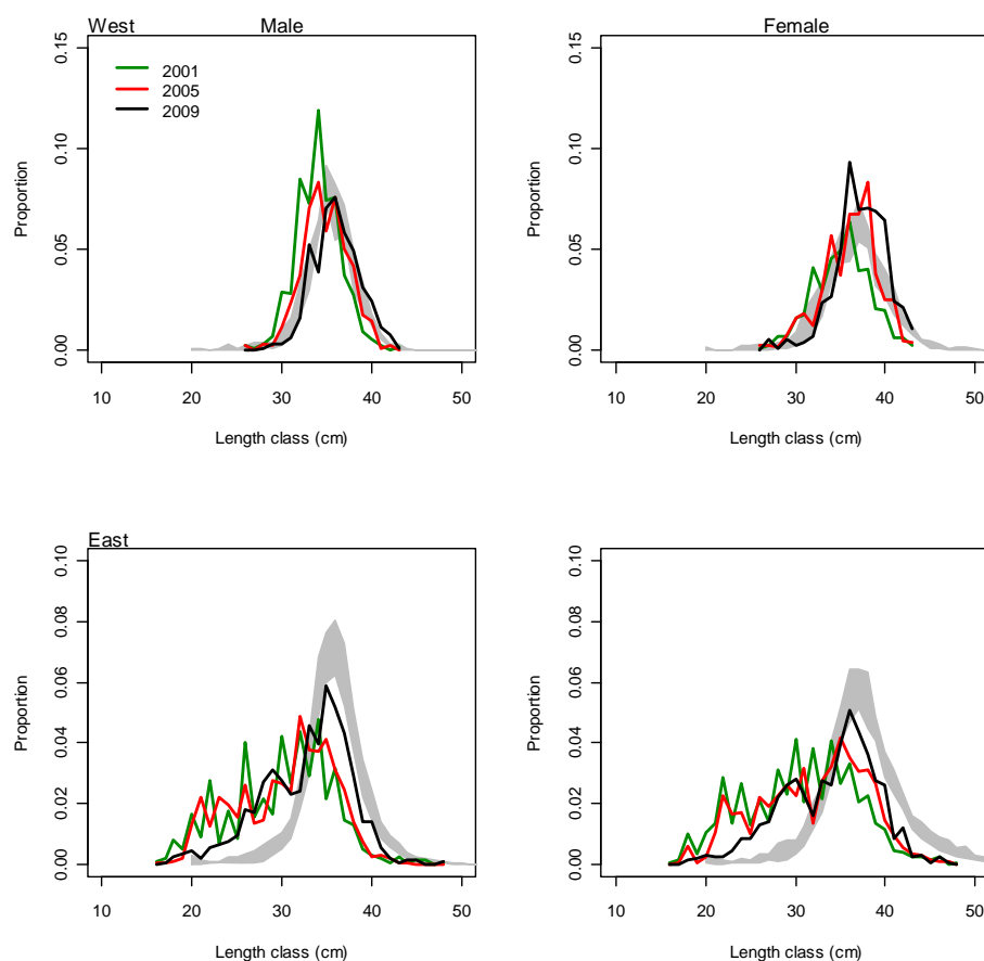
Figure 13: 2001, 2005, and 2009 acoustic survey smooth oreo length frequencies for male and female and for east and west. Shaded area represents an approximate inter-quartile region for available annual observer length frequencies.
